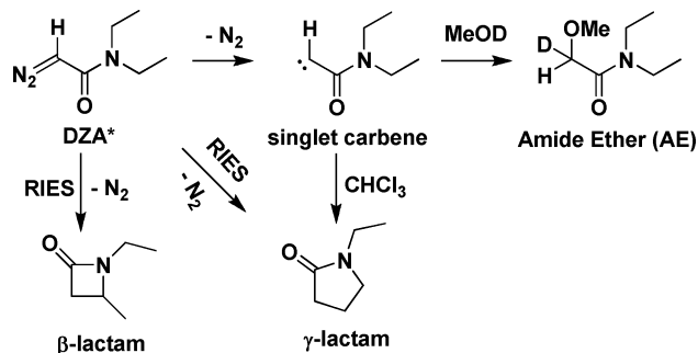
Scheme 1. Reaction Pathway for N,N -Diethyldiazoacetamide (DZA) upon Photolysis
