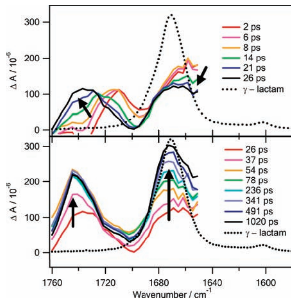
Figure 1. Transient IR spectra produced upon 270 nm photolysis of DZA in chloroform. The dashed curves are the FTIR spectra of authentic \gamma -lactam.
